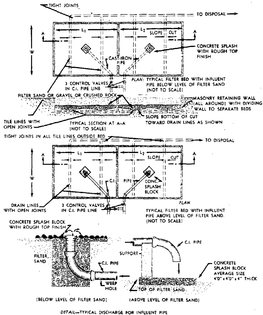
Figure 28.—Open-filter-bed layout.
