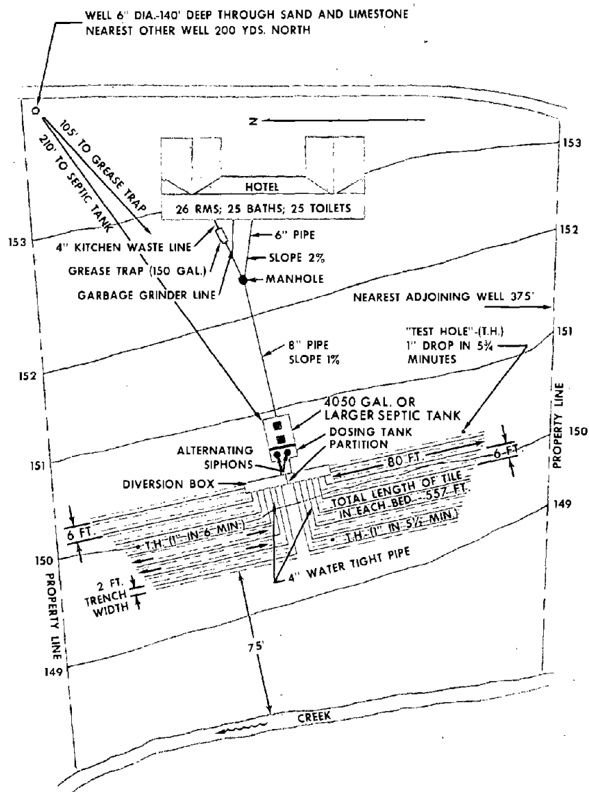
Figure 24.—Typical layout plan of a subsurface sewage-disposal system.
