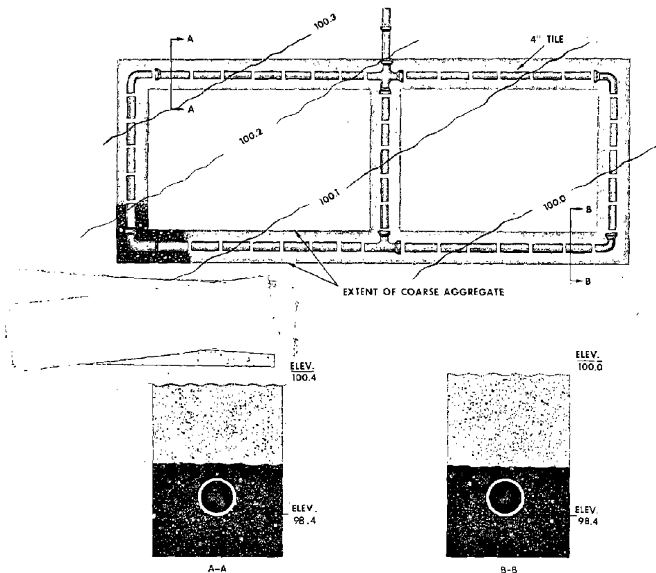
Figure 6.—Absorption-field system for level ground.
