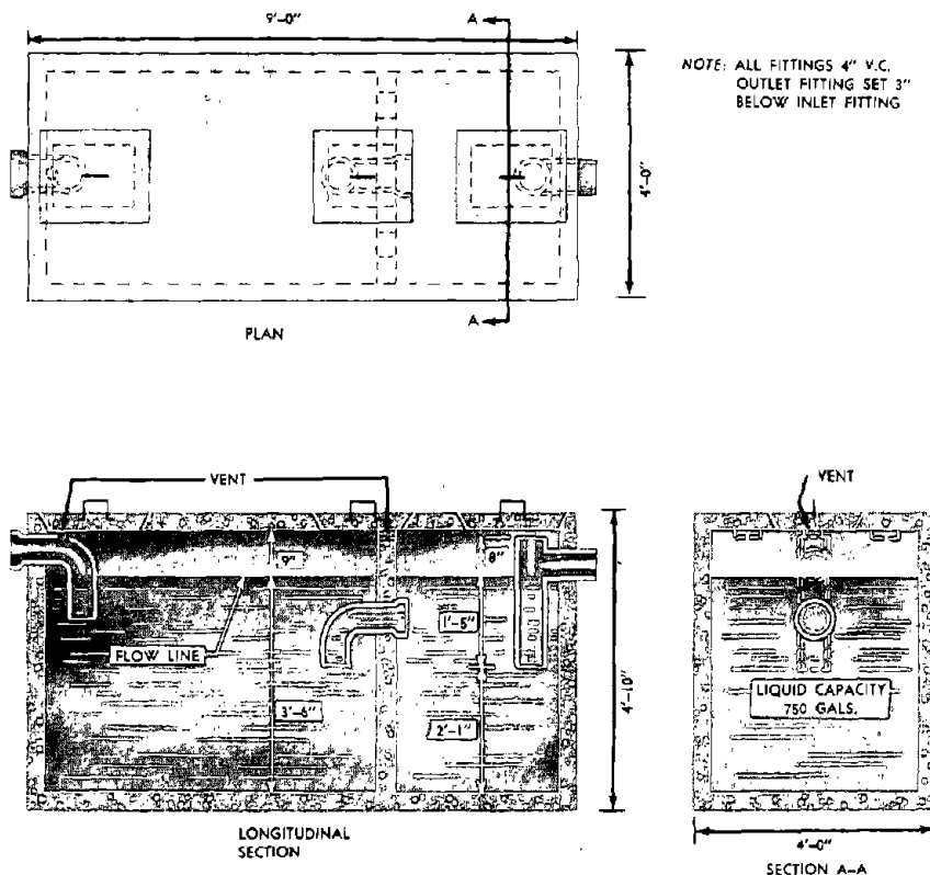
Figure 17.—Precast septic tank.
