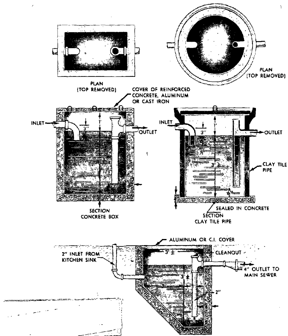
Figure 20.—Typical grease traps.
