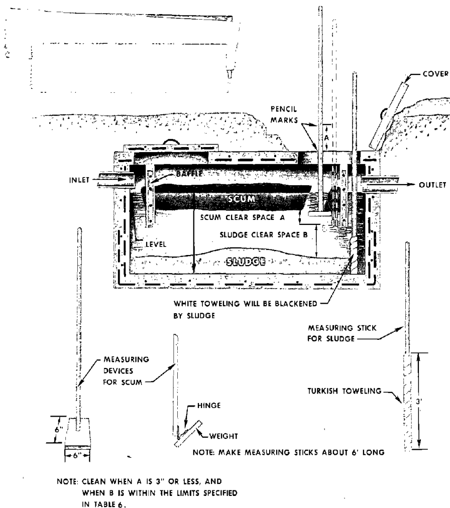
Figure 18.—Devices for measuring sludge and scum.
