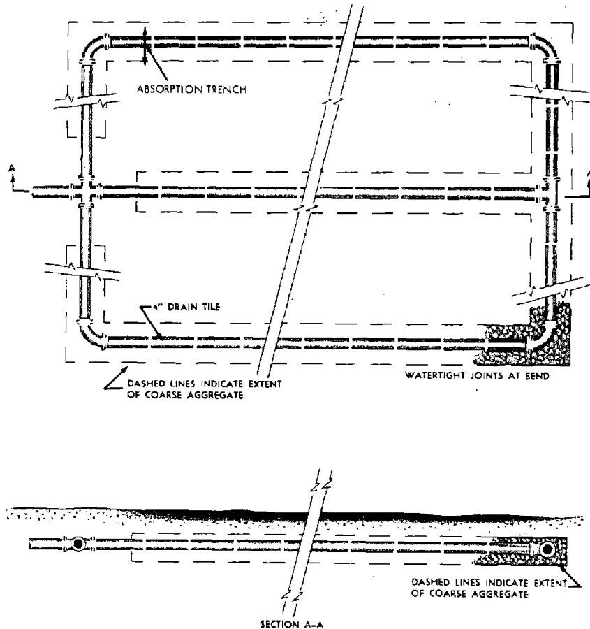
Figure 4.—Typical layout of absorption trench.
