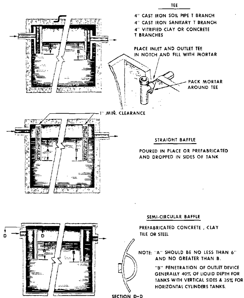
Figure 16.—Types of inlet and outlet devices.
