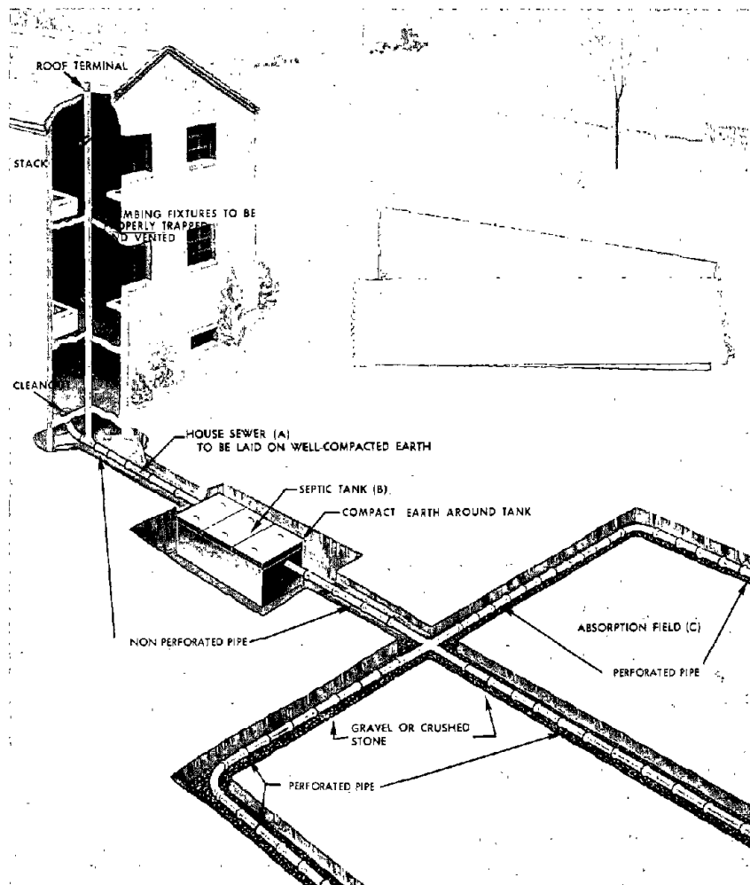
Figure 11.—Septic-tank sewage-disposal system.
