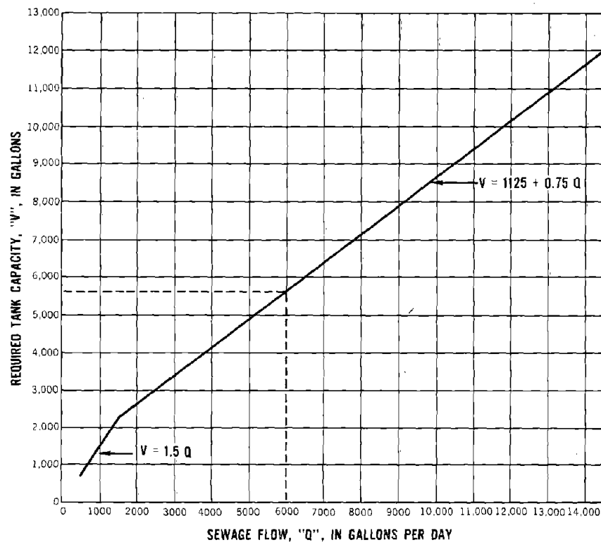
Figure 22.—Septic-tank capacities for sewage flows up to 14,500 gallons per day.
