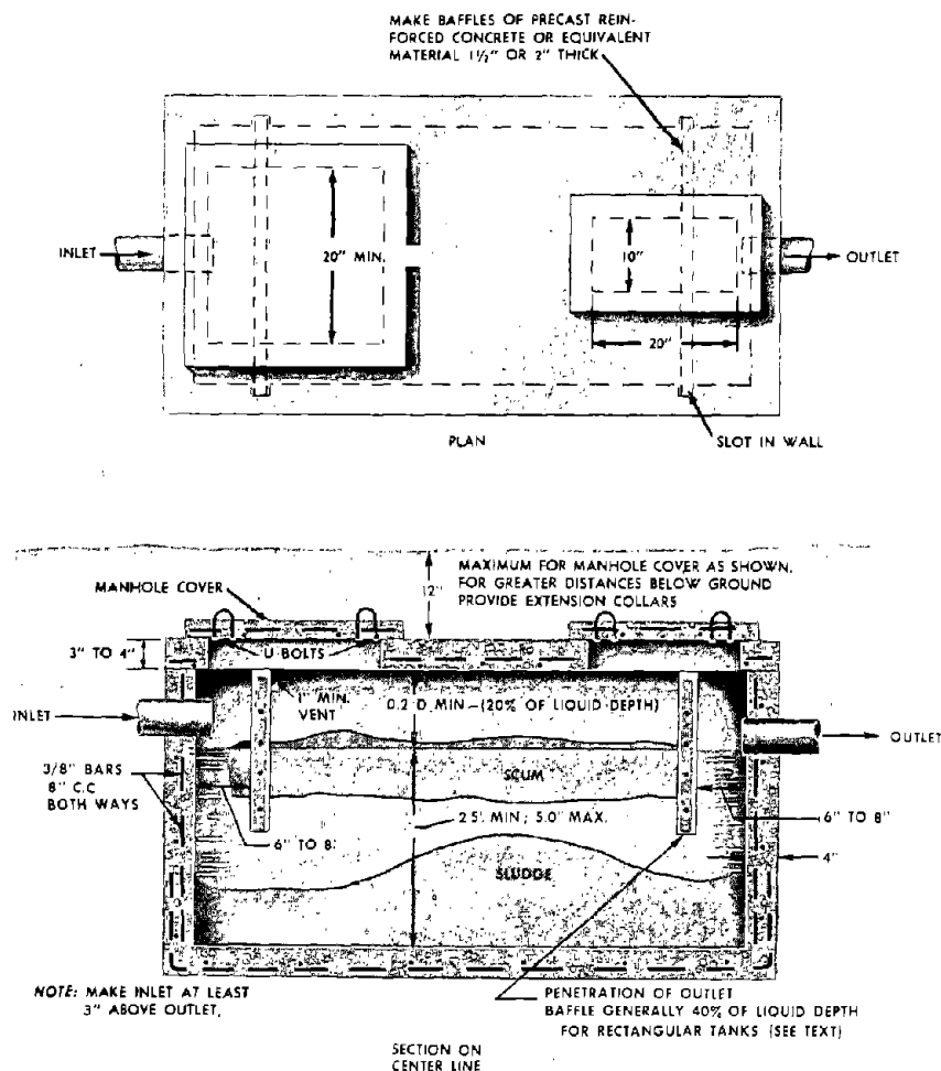
Figure 15.—Household septic tank.
