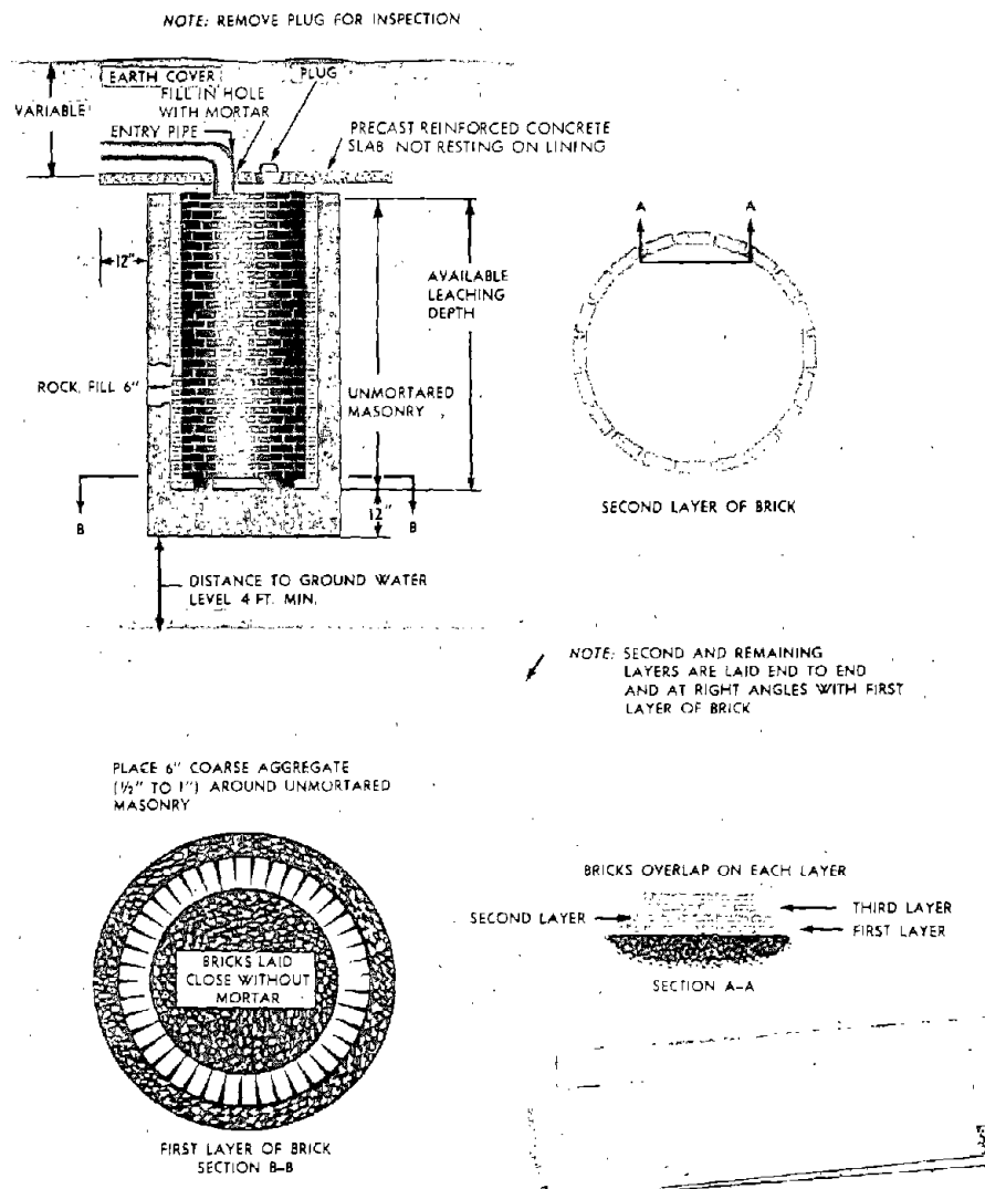
Figure 10.—Seepage pit.
