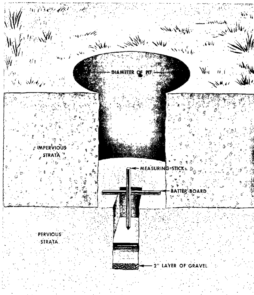
Figure 8.—Deep percolation test for seepage pit.
