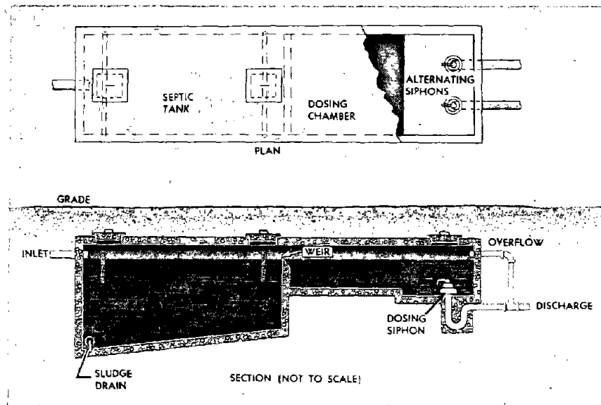
Figure 23.—Septic tank and dosing tank with alternating siphons.
