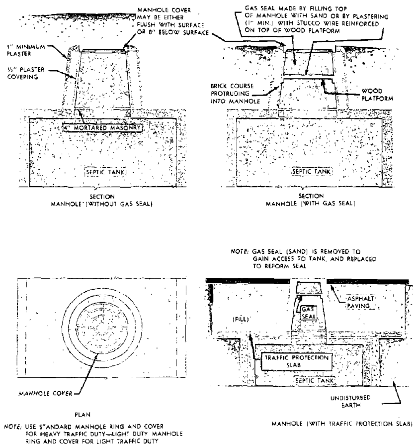
Figure 14.—Design of manholes.
