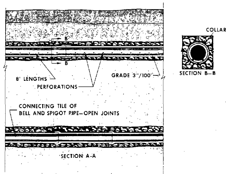
Figure 26.—Underdrained sand-filter trench.
