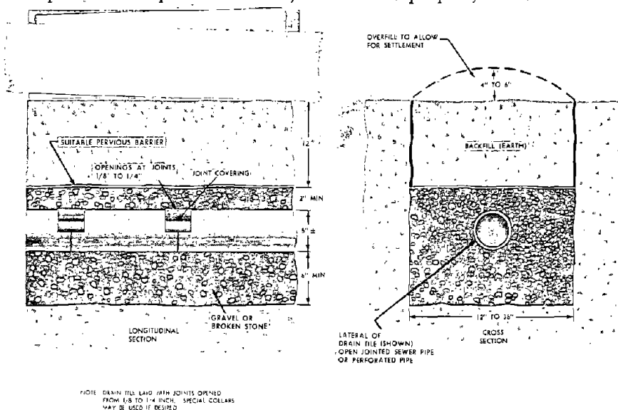
Figure 5.—Absorption trench and lateral.
