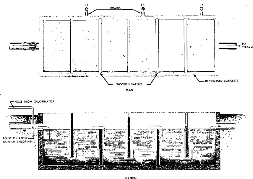
Figure 29.—Chlorine-contact chamber.
