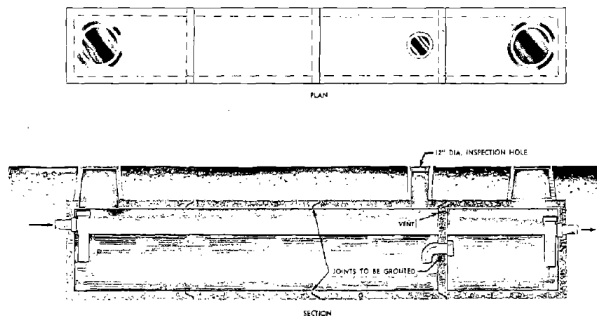
Figure 21.—Battery of four precast reinforced-concrete septic-tank sections.
