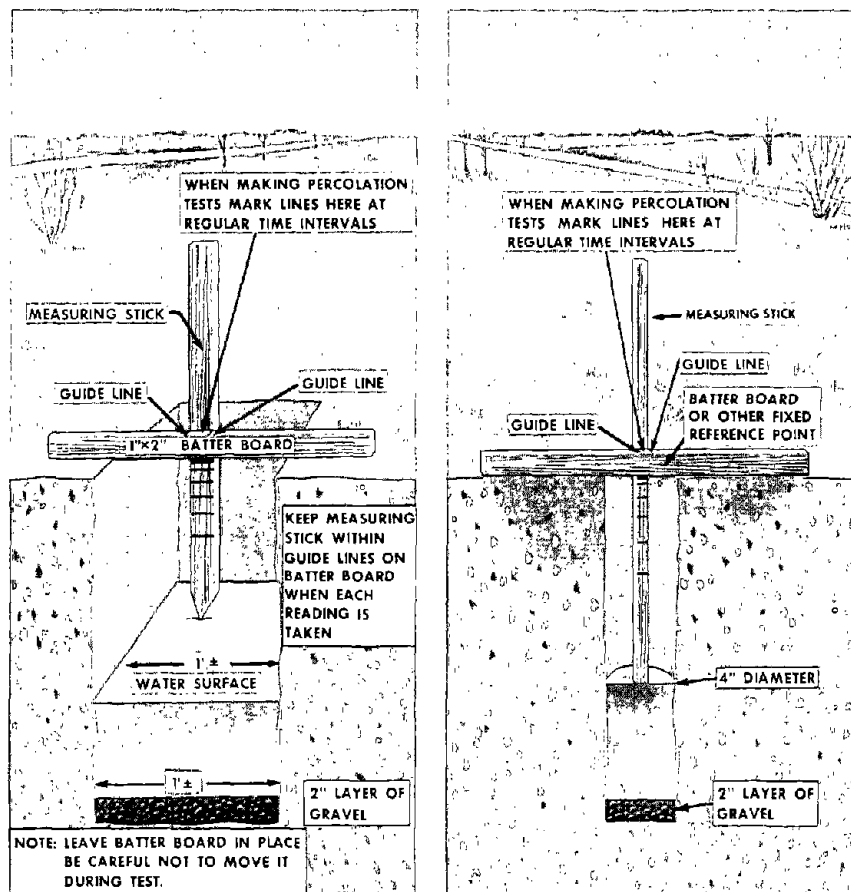
Figure 2.—Methods of making percolation tests.
