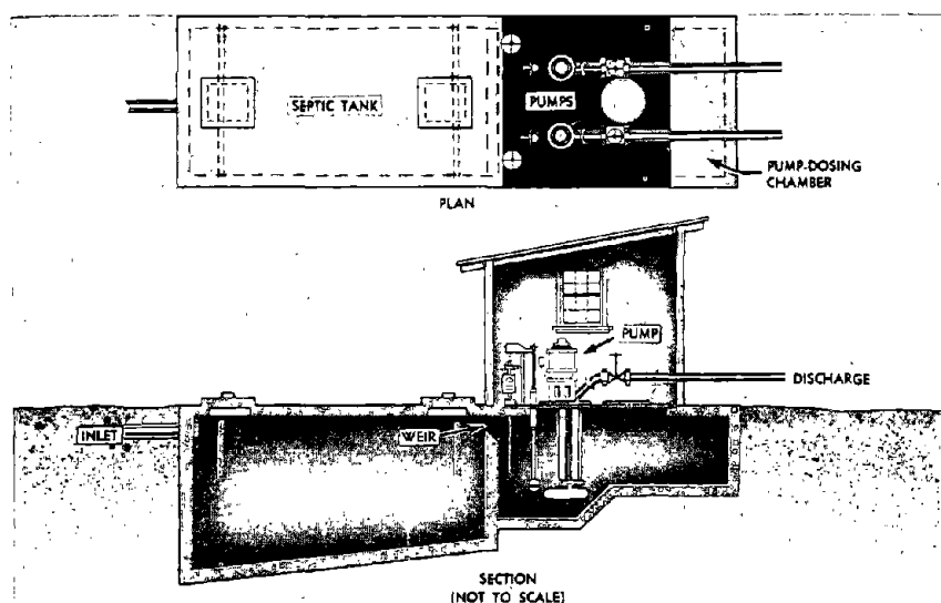
Figure 25.—Septic tank and pump-dosing chamber.
