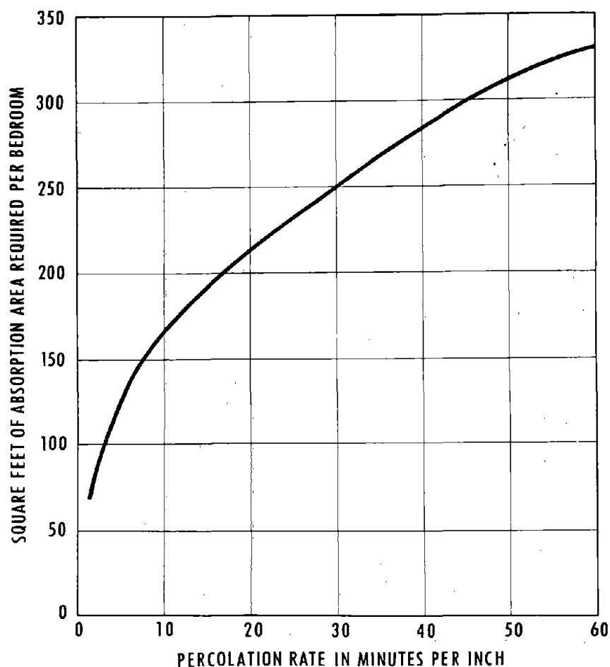
Figure 3.—Absorption area requirements for private residences.
