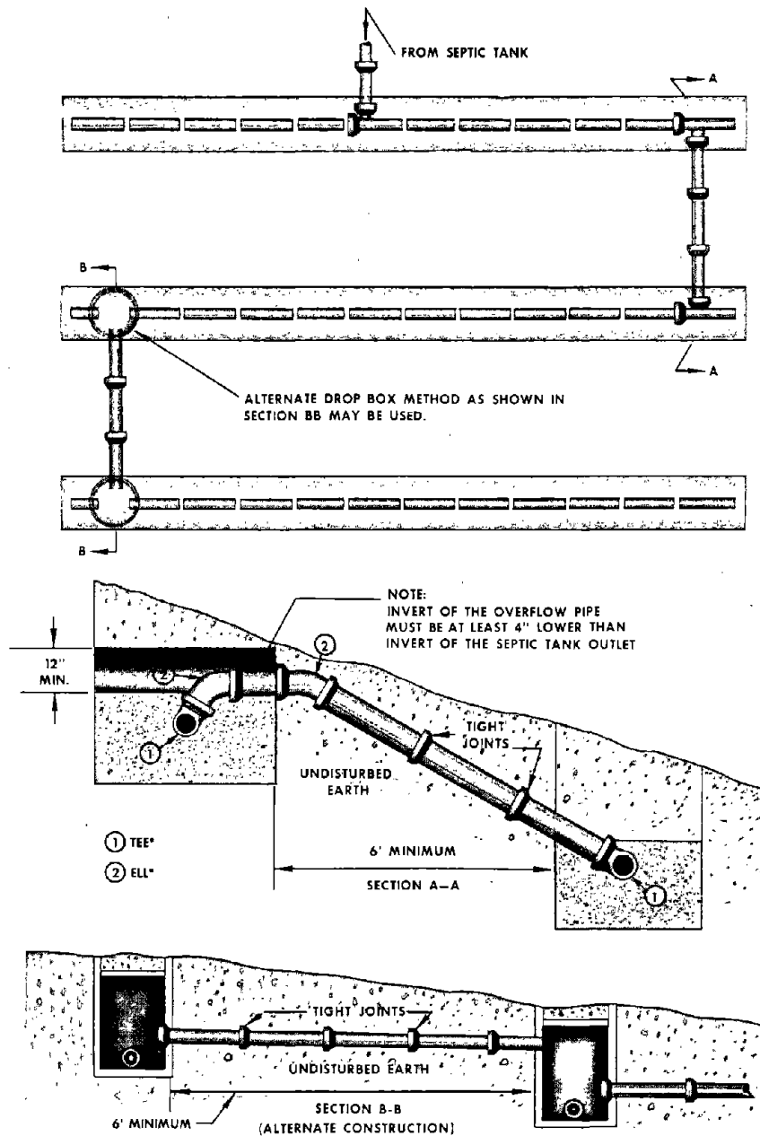
Figure 7.—A relief line arrangement for serial distribution.
