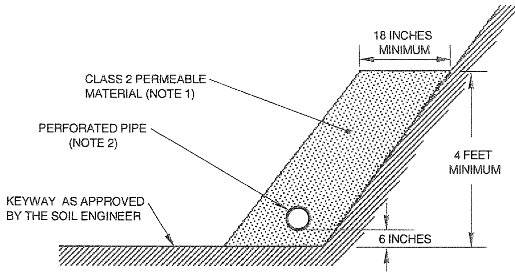
KEYWAY SUBDRAIN
