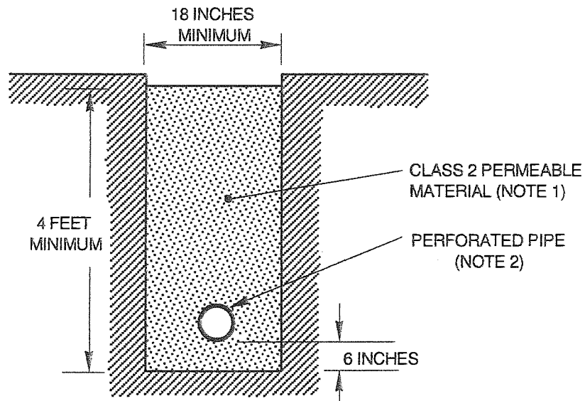
COLLECTOR SUBDRAIN
